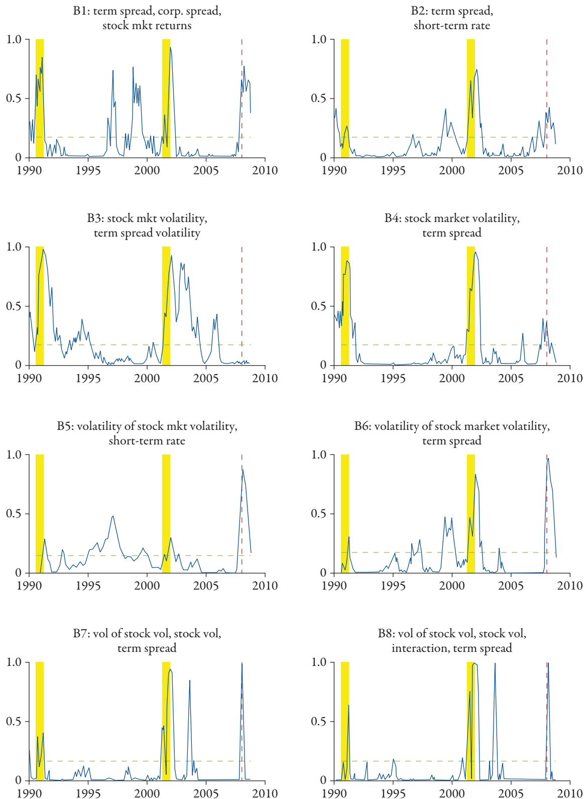
Figure 6: Probabilities of recession predicted by Probit models: out-of-sample, coincident projections.
