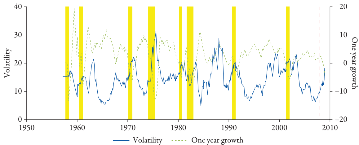
Figure 1: Aggregate stock market volatility and industrial production growth.
