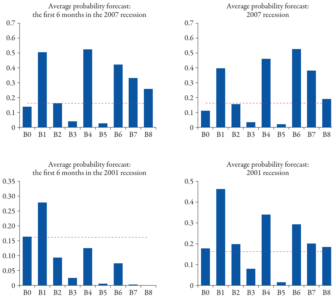
Figure 8: A tale of two recessions, 2001 and 2007: average probabilities of recessions predicted by Probit models, out-of-sample, six month projections.
