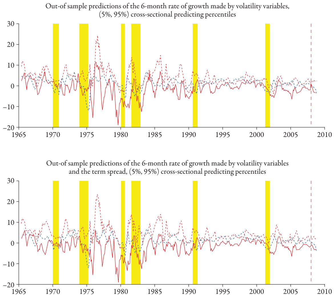
Figure 5: Linear predictions of economic activity.
