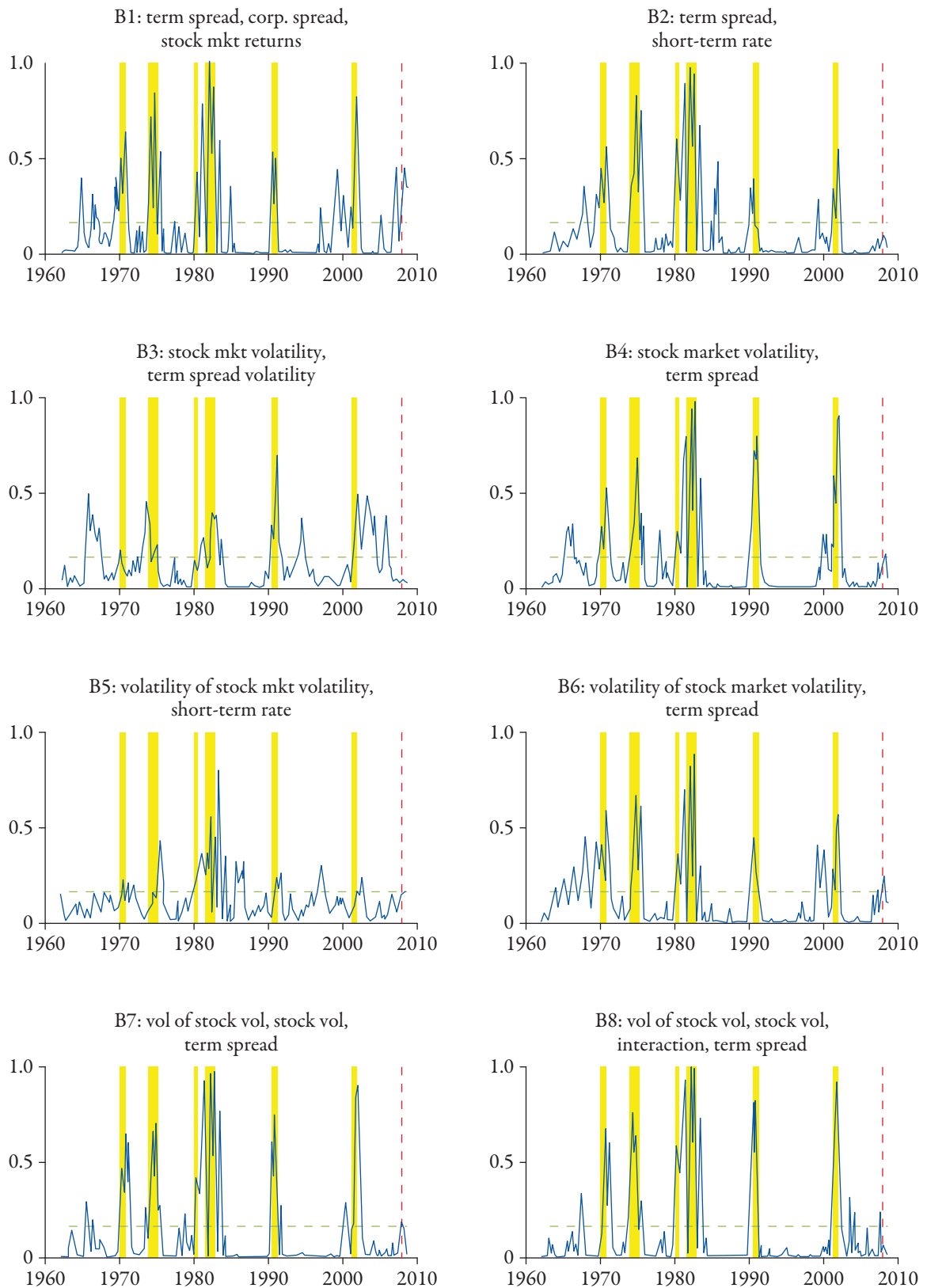
Figure 4: Probabilities of recession predicted by in-sample estimates of Probit models.
