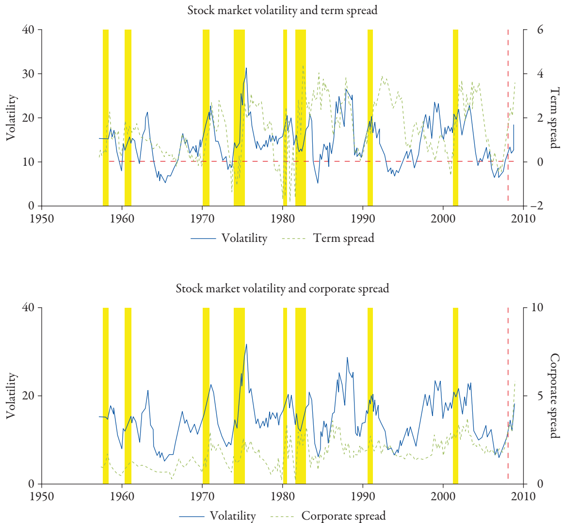
Figure 2: Aggregate stock market volatility, the term spread and the corporate spread.
