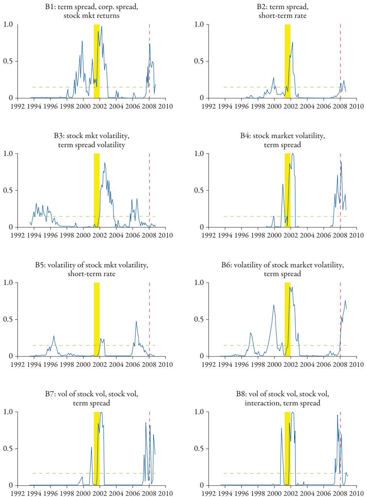
Figure 7: Probabilities of recession predicted by Probit models: out-of-sample, six month projections.
