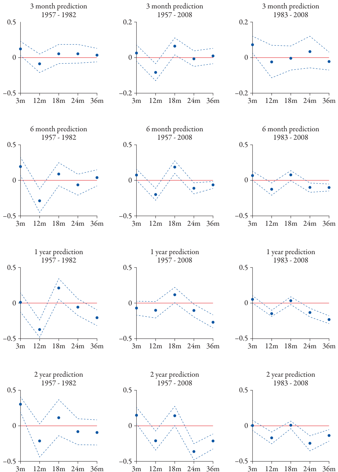
Figure 3: Estimates of volatility loading on industrial production growth.
